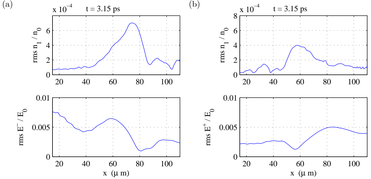
Figure 5-5: rms n_1 = n_e - n_e(t=0) and reflected light for inhomogeneous runs with L_n=167 \mu\text{m} and (a,b) k_0||(+, -)\nabla n . The E^- and E^+ signals are filtered to only pass the band from k\lambda_D = 0.07 - 0.19 , which includes the SRS seed.
