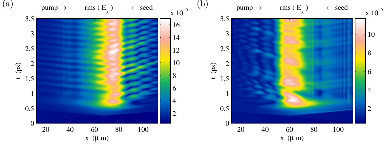
Figure 5-4: rms E_x for inhomogeneous run with L_n=167 \mu\text{m} and (a,b) k_0||(+, -)\nabla n . The pulsations continue for the rest of the runs (total time 7 ps).
