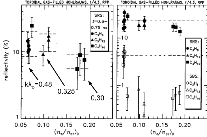
Figure 1-3: Experimental results from Fig. 5 of [11], showing a flight increase of SRS reflectivity with k\lambda_D of the EPW.
