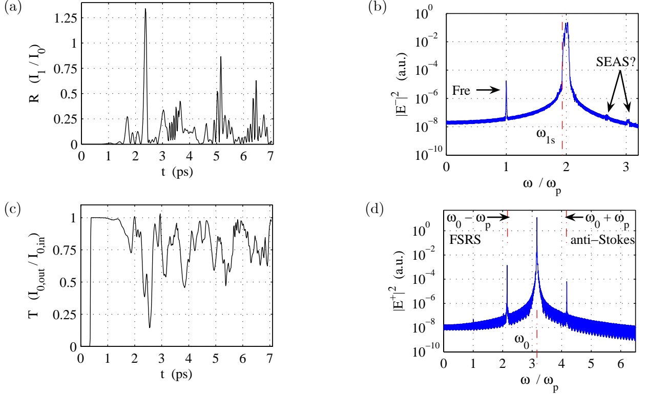
Figure 3-2: (a) Reflectivity R and (b) gated E^-(x=0) spectrum over the whole run BC1. “Fre” and “SEAS?” denote forward re-scatter of BSRs light and possible stimulated electron acoustic scatter, respectively. \omega_{1s} is the seed scattered light frequency. (c) Transmitted fraction T and (d) gated E^+(x=L) spectrum over whole run at right edge.
