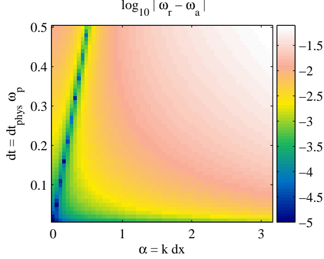
Figure A-4: Phase error for the Langdon-Dawson method used to advance the transverse fields v_{ye} and E^\pm . The error becomes large exactly at \alpha = \pi (not shown; the abscissa ends at \alpha = 3.14 ).
