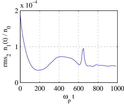
Figure A-5: Density perturbation n_1 = n_e - n_0 near box center for run ES .
