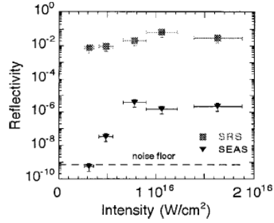
FIG. 10. Plot of measured reflectivity in SRS and SEAS vs laser intensity. SEAS reflectivity drops below detection level for I \leq 3 \times 10^{15} W/cm², and is \sim 3000\times below the SRS levels for higher intensity.
