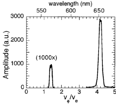
FIG. 9. Plot of SEAS and SRS backscatter spectrum vs electrostatic wave v_\phi/v_e for single hot spot experiment. SEAS mode is shown 1000× larger. Upper axis corresponds to the scattered light wavelength.
