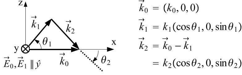
Figure 2-1: Fluid model geometry. Light waves polarized perpendicular to k -plane.
